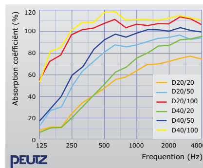
Sound absorption values
